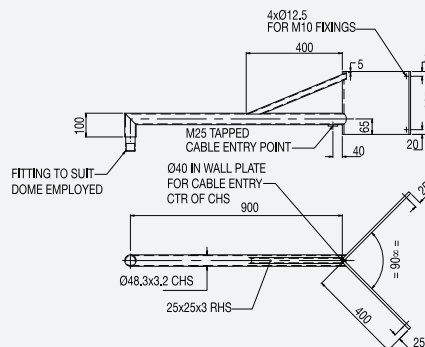
Corner mount standard CB2-900-D
