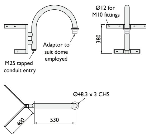
C-1699/F Corner mount
