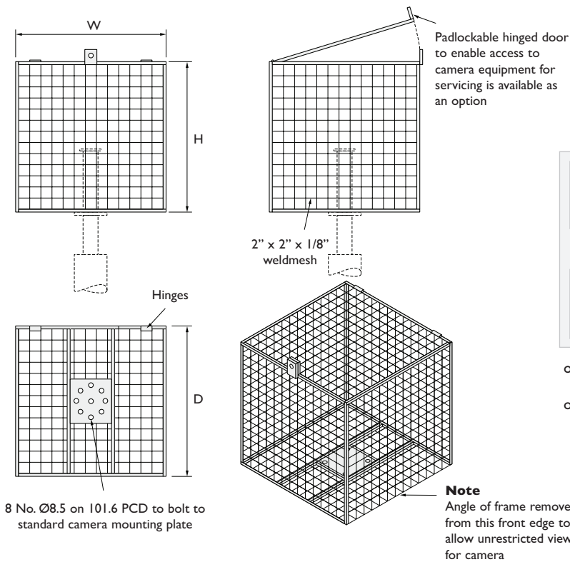
Pole top mounted cage
